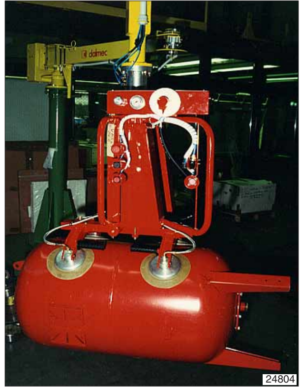
Manipulator with suction cups tooling (Venturi) for gripping and inclination of tanks.
